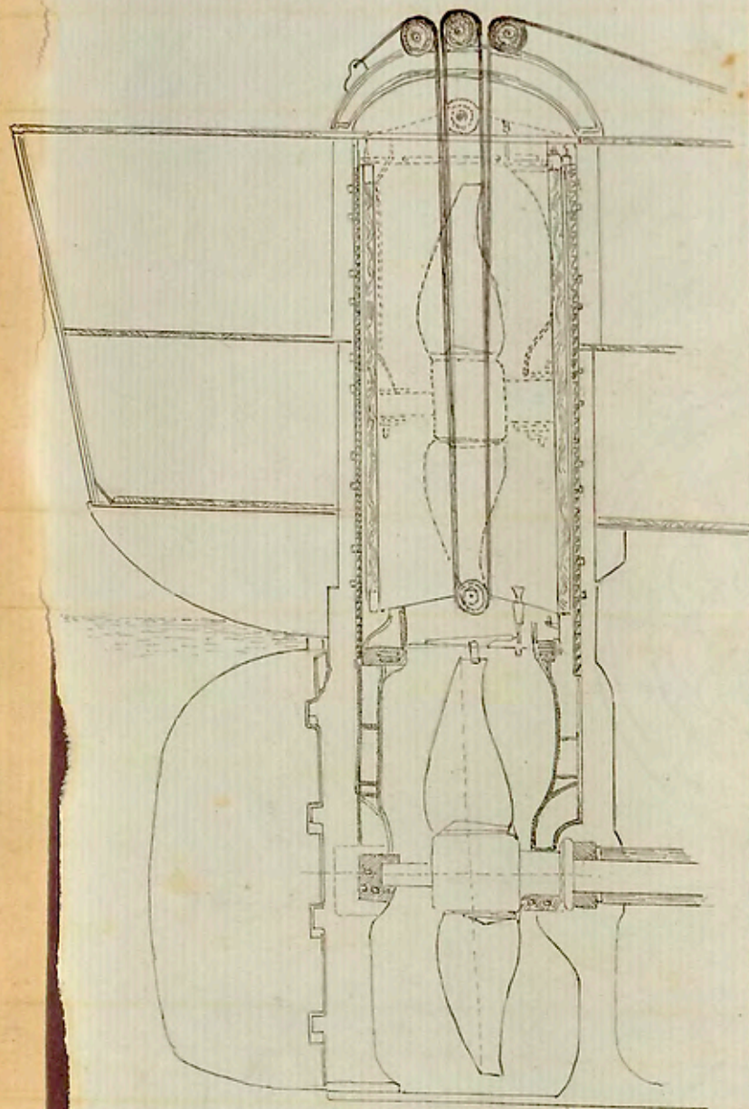
PLAN OF RAISING SCREW
